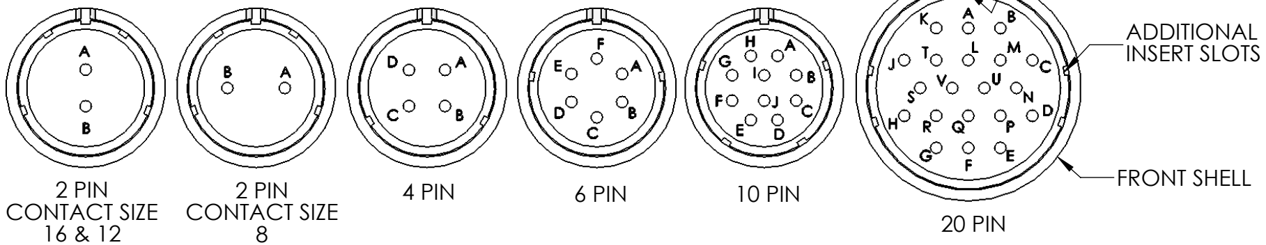
FIG 6 VIEW A-A
