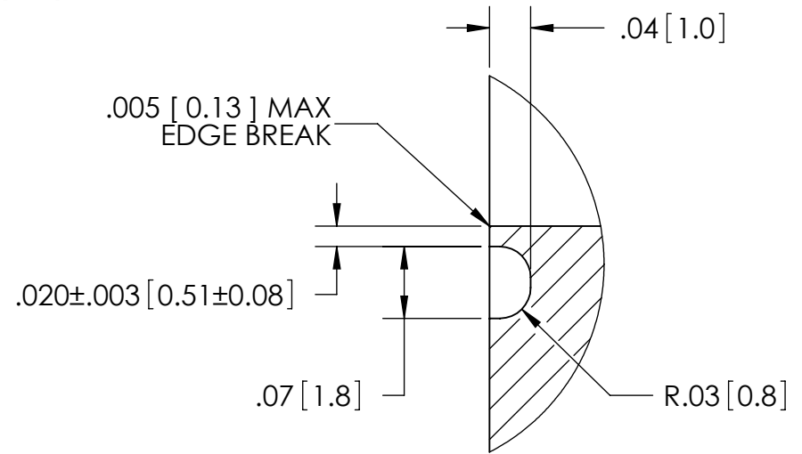
DETAIL B SCALE 6 : 1
